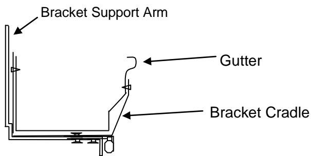
Rotating Bracket with Gutter Installed
